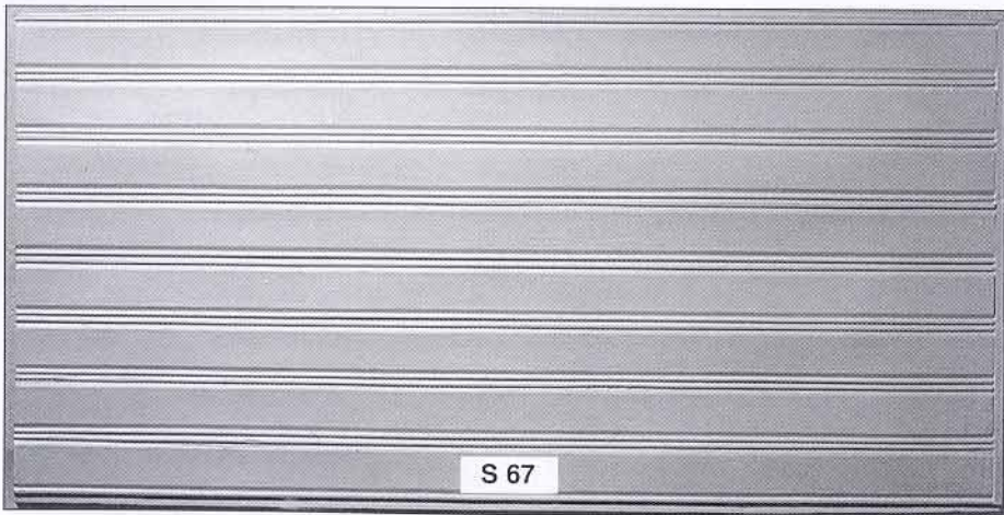
Match boarding with bead and flute Panel size: 2135 x 1055 x 6 mm
