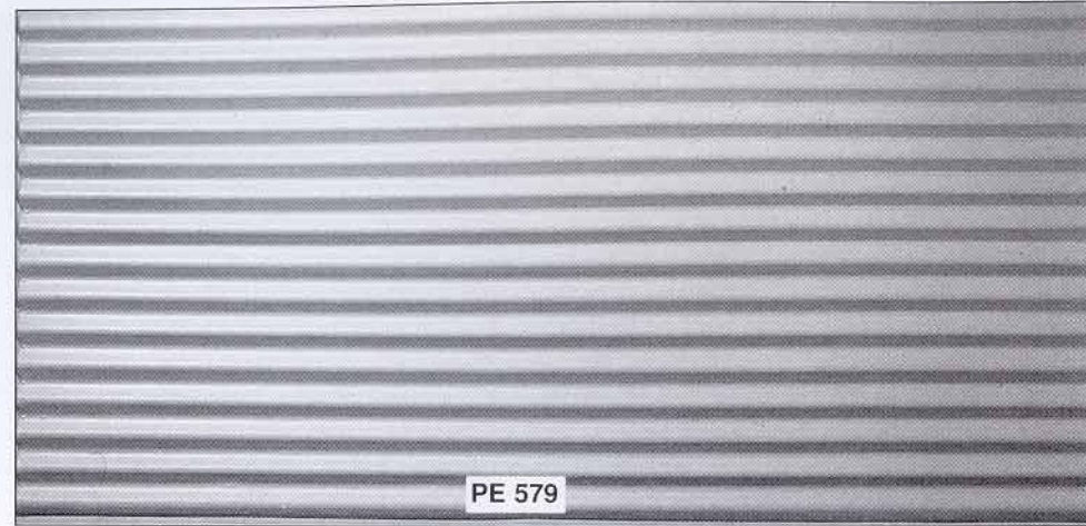
Corrugated iron - 76 mm Pitch Panel size: 2400 x 1100 x 20 mm
