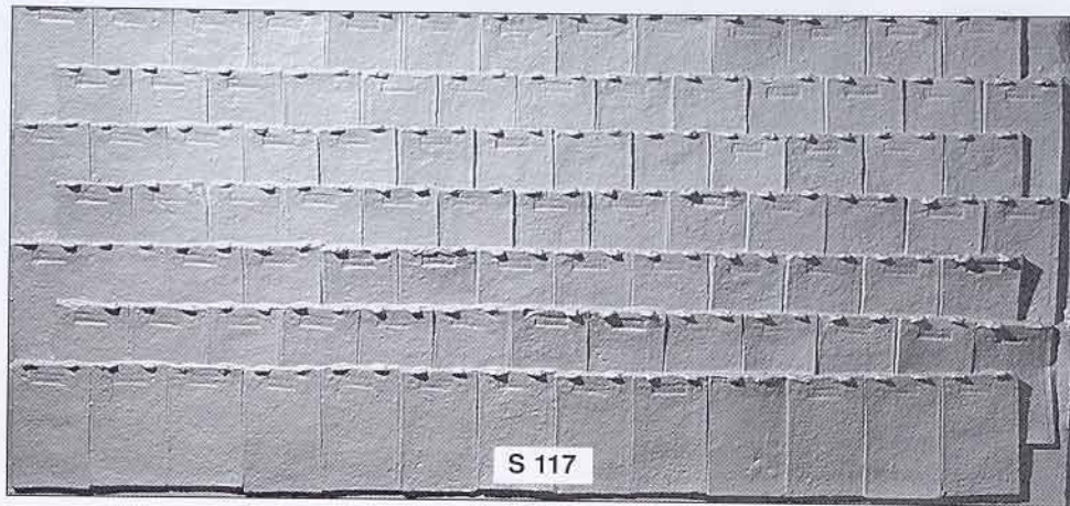
Underside of roofing tiles - Tile size: 135 x 165 mm Panel size: 2285 x 1040 x 25 mm
