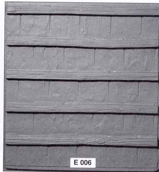
Slates underside Panel size: 1137 x 1110 x 38 mm
