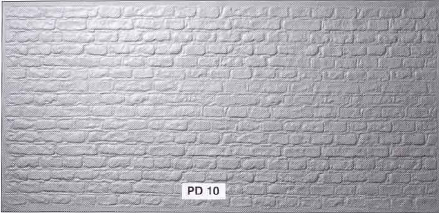
Cottage small brickwork Brick size: 200 x 50 mm Panel size: 2170 x 1020 x 8 mm
