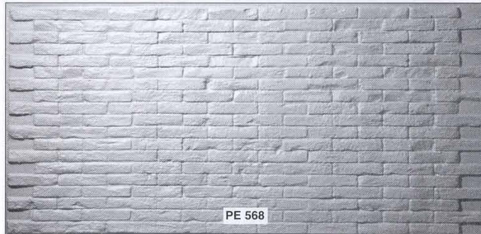
Stretcher bond brickwork Brick size: 245 x 55 mm Panel size: 2370 x 1130 x 20 mm Corner section available: PE 569 - 1780 x 350 x 350 mm
